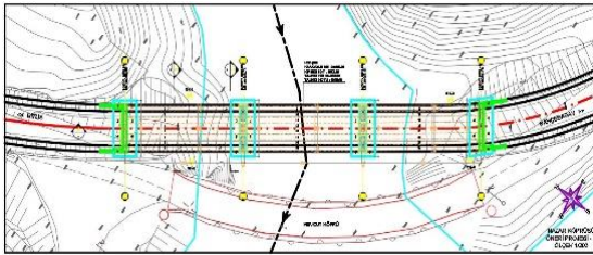
Nazar (Plan)
